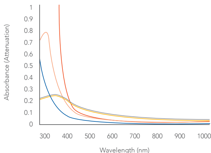
Absorbance Spectra of UV Filter Concentrates: 0.001% Active \text{TiO}_2 Diluted in C12-15 Alkyl Benzoate 1 cm Path Length
