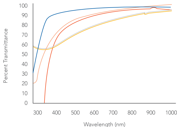
Transmittance Spectra of UV Filter Concentrates: 0.001% Active \text{TiO}_2 Diluted in C12-15 Alkyl Benzoate 1 cm Path Length
